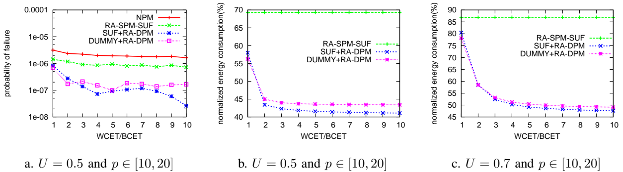
Fig. 6. Performance of the integrated schemes with 20 tasks.
