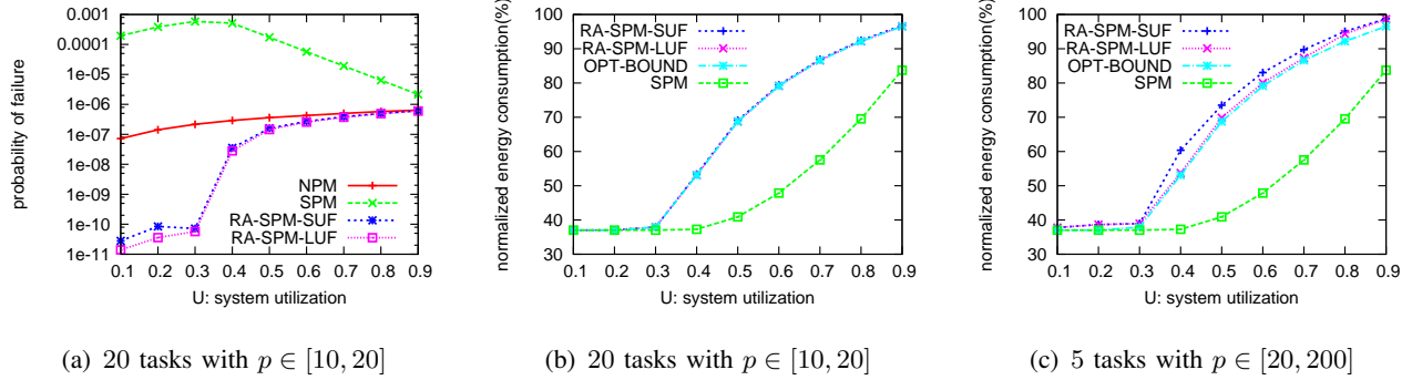
Fig. 3. Reliability and energy consumption for static schemes.
