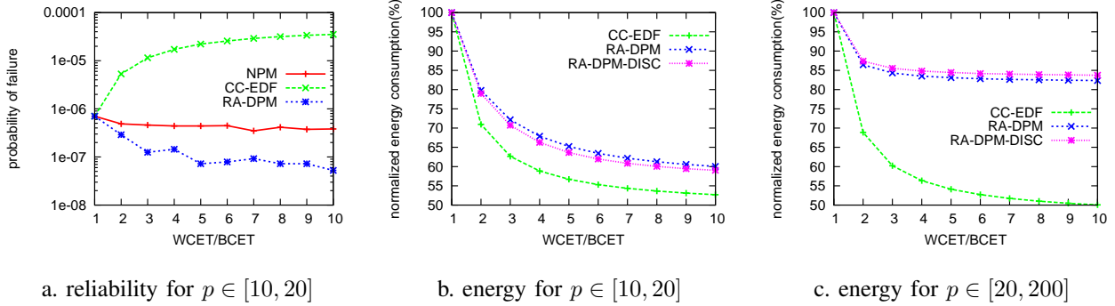
Fig. 4. Reliability and energy consumption for dynamic schemes.
