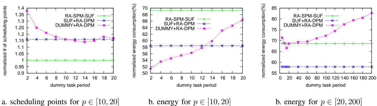
Fig. 5. Effects of the dummy task's period. Here, U = 0.5 and \frac{WCET}{BCET} = 1 .
