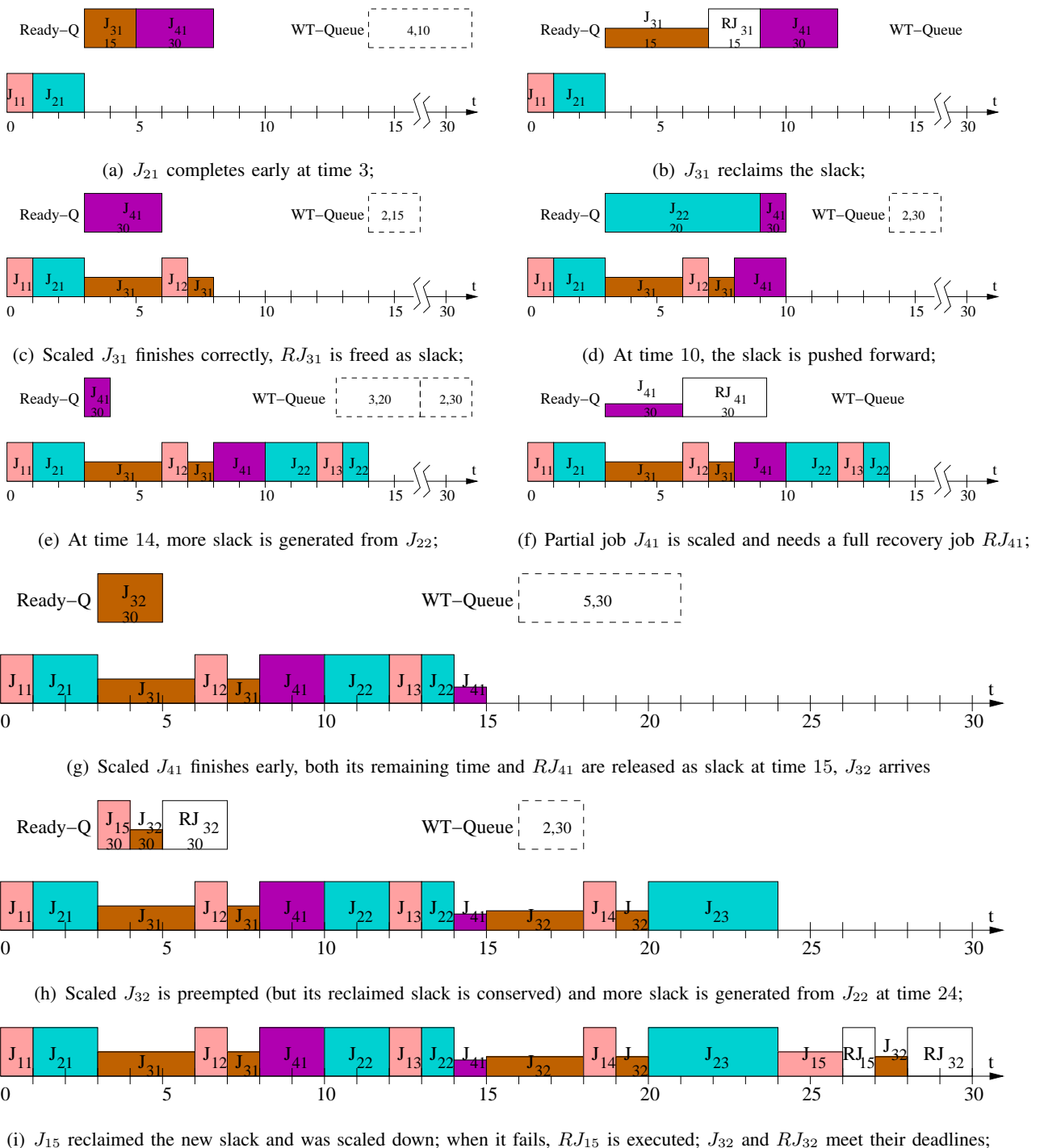
Fig. 2. Using wrapper-tasks to manage dynamic slack.
