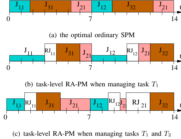
Fig. 1. Static schemes for a task set with three tasks \{T_1(1, 7), T_2(2, 14), T_3(2, 7)\} .
